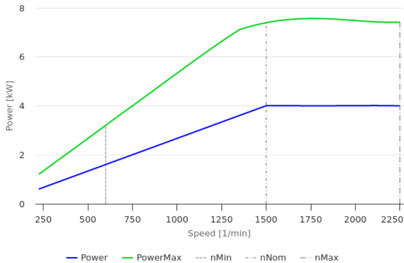
Power-Speed-Curves 4)
