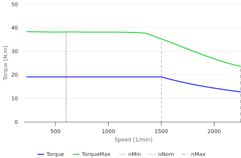
Torque-Speed-Curves 4)
