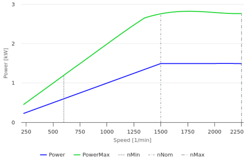
Power-Speed-Curves 4)
