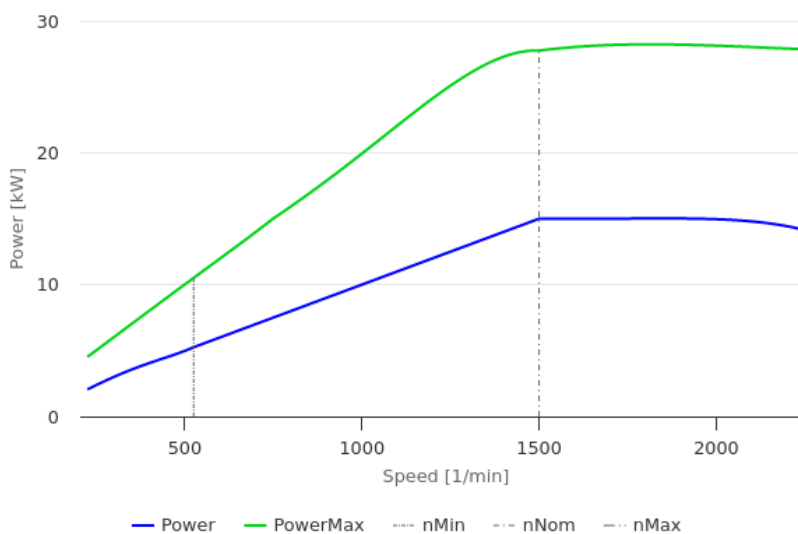
Power-Speed-Curves 4)
