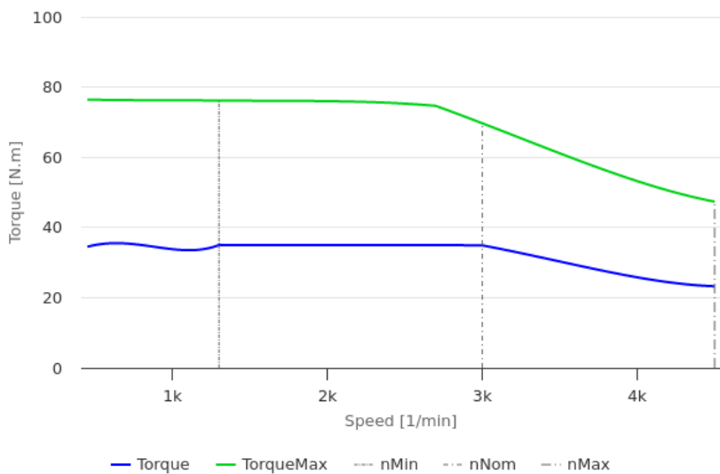
Torque-Speed-Curves 4)
