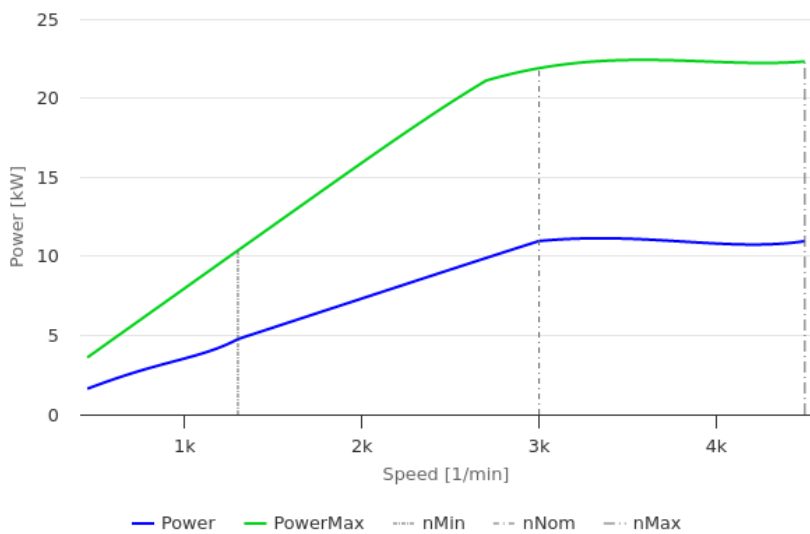
Power-Speed-Curves 4)
