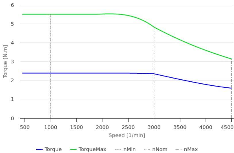
Torque-Speed-Curves 4)
