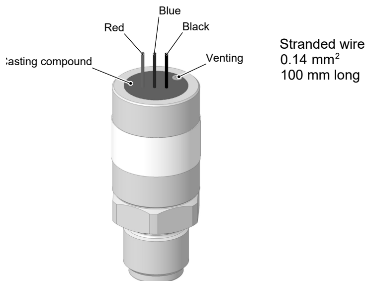
Fig. 3: Electrical connection options
