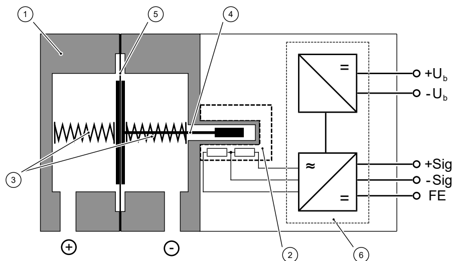
Fig. 1: Function diagram
