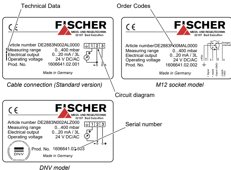
Fig. 3: Nameplate
