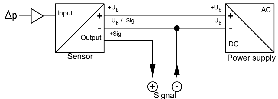
Fig. 6: 3-conductor circuit
