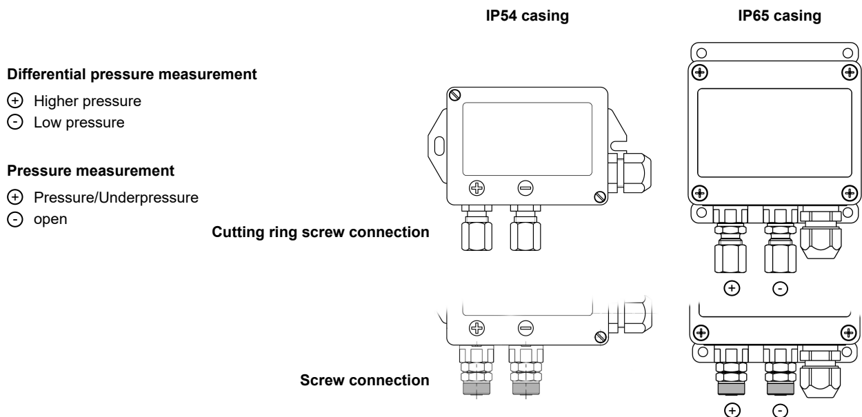
Fig. 5: Process connection
