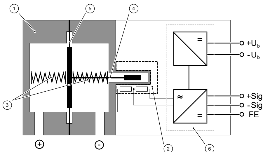
Fig. 4: Function diagram
